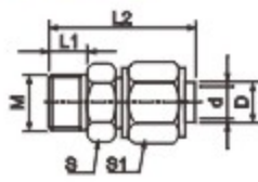
FN-直通终端管接头 FN-Male stud
