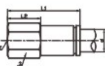
FCR-B 内螺纹接头 FCR-B Female stud
