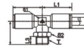
FCR-Y 三通边部螺纹接头(360° 旋转) FCR-Y Male stud run tee(360° circumrotation)
