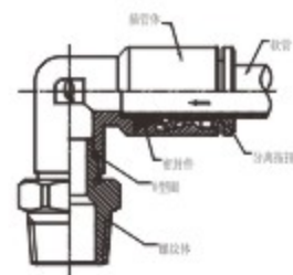
FCR-L 直角螺纹接头(360° 旋转) FCR-L Male stud elbow(360° circumrotation)
